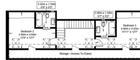
Second Floor
