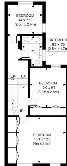
SECOND FLOOR GROSS INTERNAL FLOOR AREA 554 SQ FT
