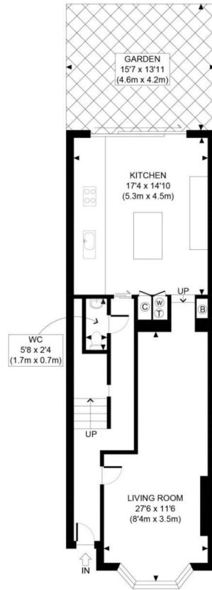
GROUND FLOOR GROSS INTERNAL FLOOR AREA 700 SQ FT
