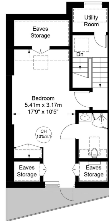
Fourth Floor
