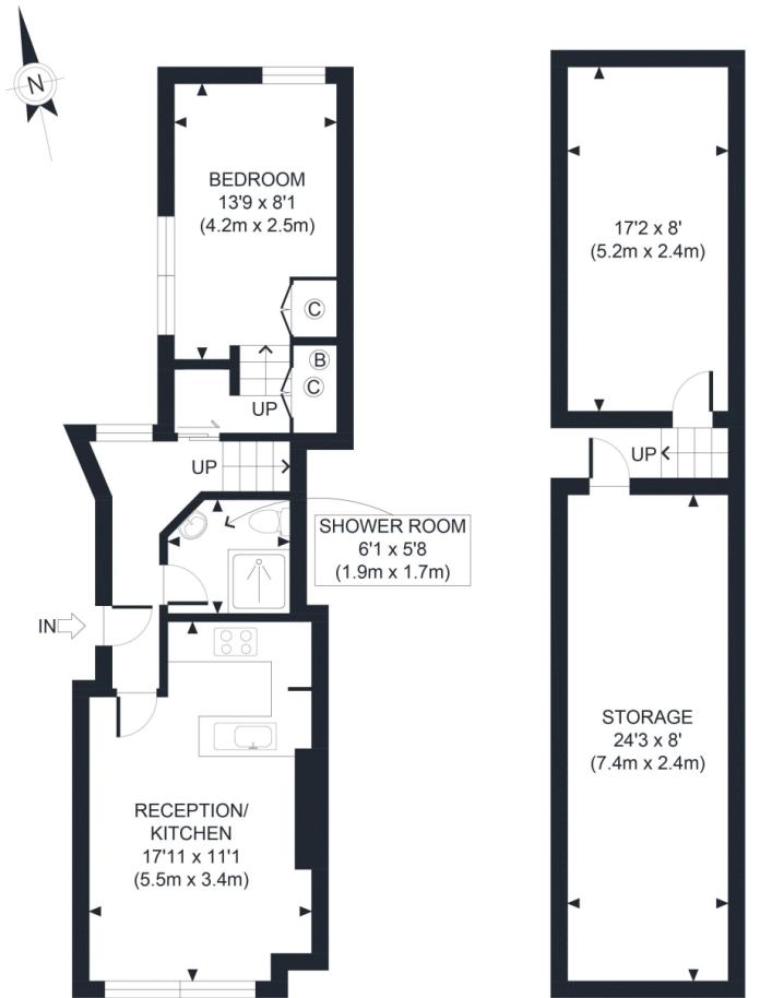
TOP FLOOR
