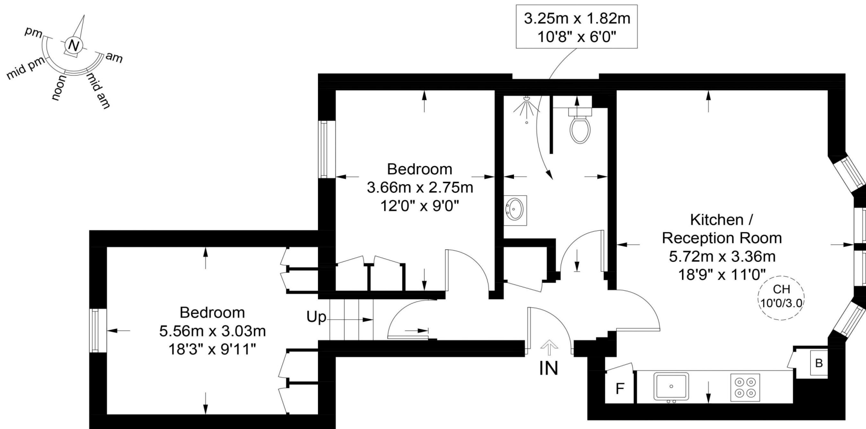
First Floor
